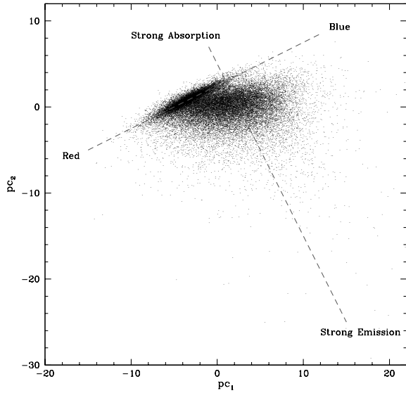
Figure 2. Projections ( pc_1 and pc_2 ) in the space defined by the first two eigenspectra derived from the PCA for the M_{bj} - 5 \log_{10}(h) < -18 sample of galaxy spectra. The trends illustrated have been derived from the eigenspectra by identifying the linear combinations that either maximize the influence of the absorption/emission features or minimize them.
