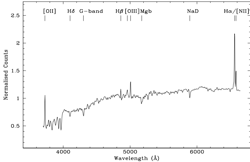
Figure 1. The average spectrum of the M_b - 5 \log_{10}(h) > -18 volume-limited sample of galaxies. The main spectral features present are labelled.
